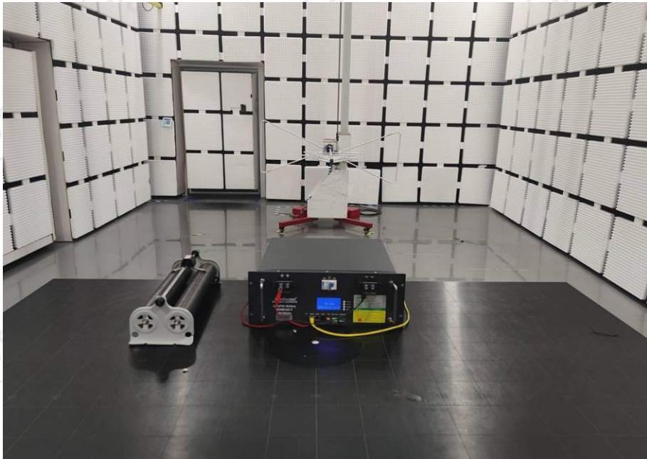
Radiated emission (30 MHz-1 GHz) test view
