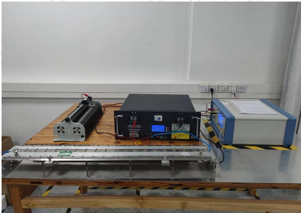
Electrical fast transient/burst immunity (EFT/B) test view
